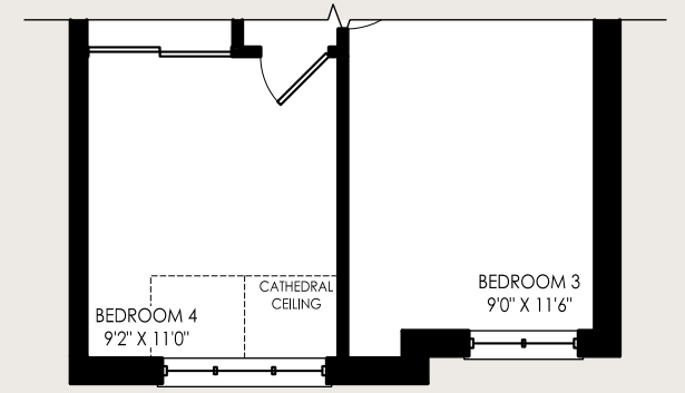
PART. SECOND FLOOR STYLE 'C'
