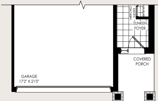
PART. GROUND FLOOR STYLE 'C'
