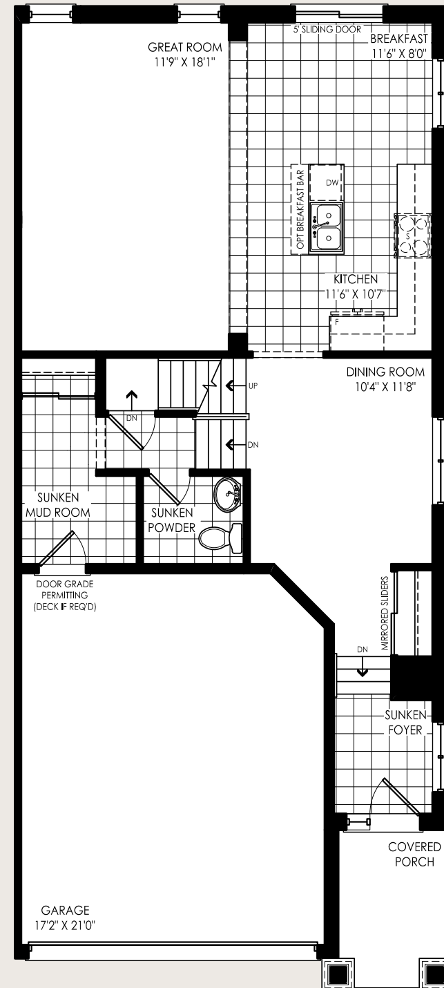
GROUND FLOOR STYLE 'A'
