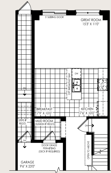
PART. OPT. GROUND FLOOR HALLWAY W/ ALT. GROUND FLOOR KITCHEN
