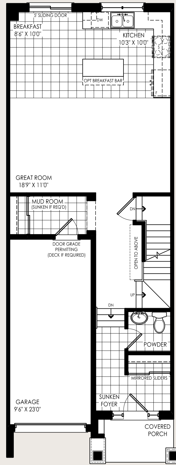
GROUND FLOOR STYLE 'A' & 'A1'
