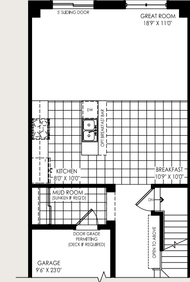
PART. ALT. GROUND FLOOR
