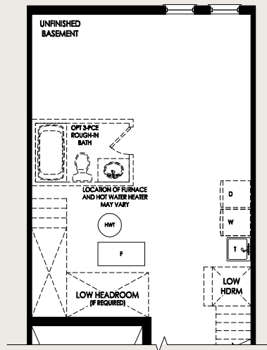
PART. BASEMENT FLOOR FOR OPT. GROUND FLOOR HALLWAY
