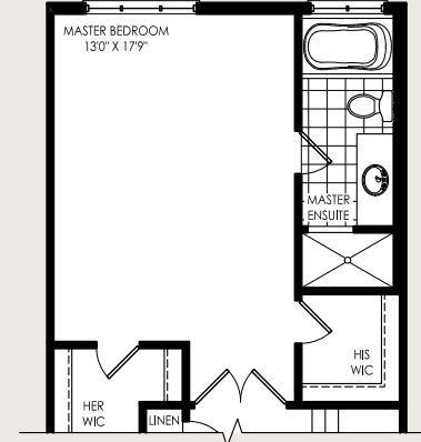
PART. SECOND FLOOR STYLE 'A' W/ OPT. 4 PC ENSUITE
