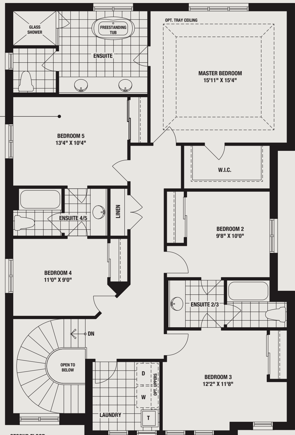
SECOND FLOOR W/OPT. 5 BEDROOM ELEV. 'A'
