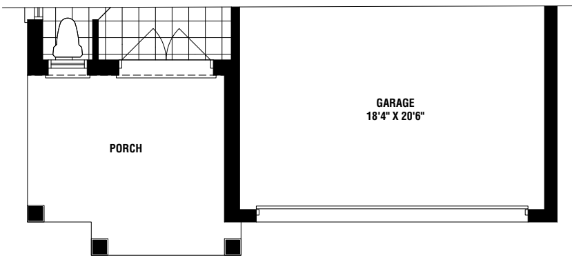
GROUND FLOOR ELEVATION 'A'
