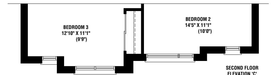
SECOND FLOOR ELEVATION 'C'
