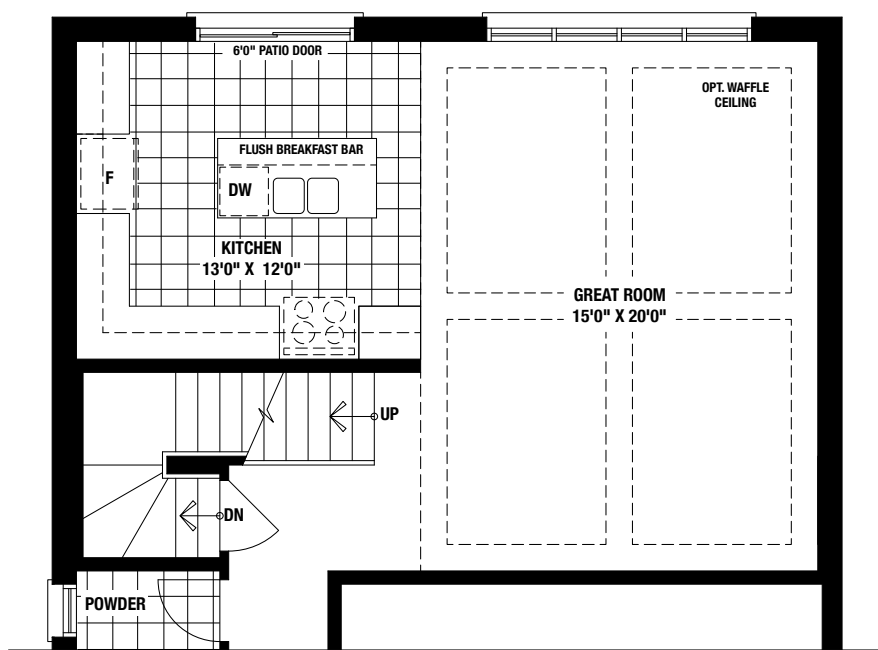
ALTERNATE MAIN FLOOR ELEVATION 'A', 'B', & 'C'
