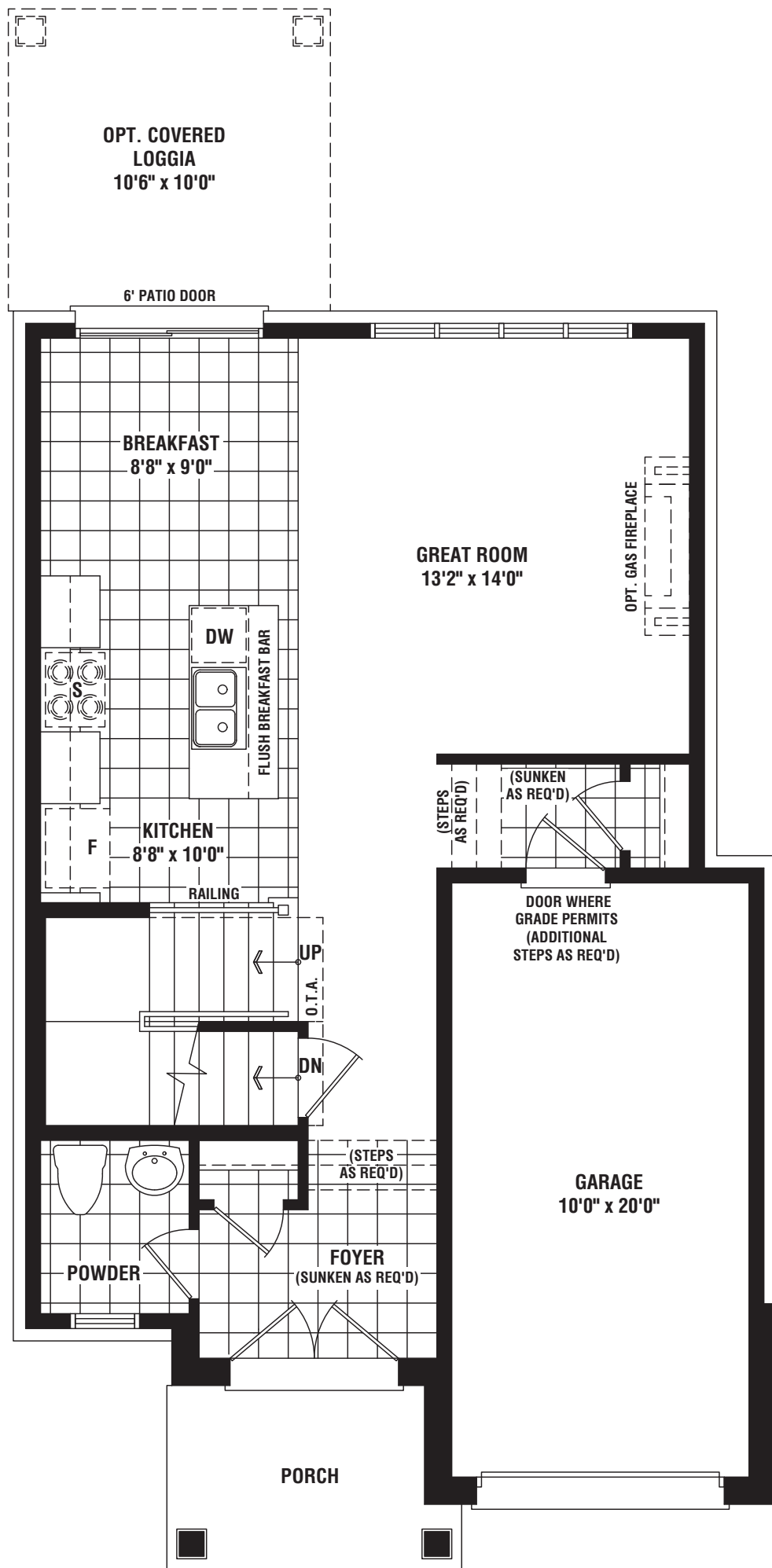
GROUND FLOOR PLAN ELEV. 'A'
