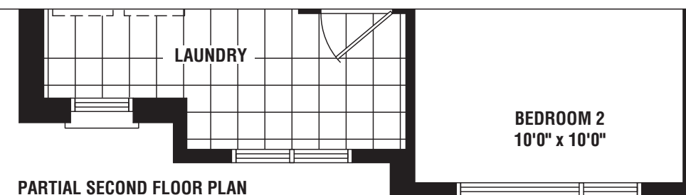
PARTIAL SECOND FLOOR PLAN ELEV. 'C'
