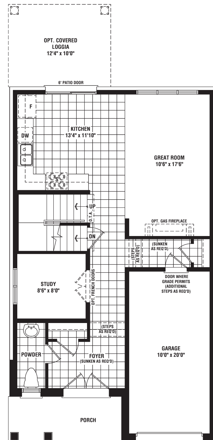
ALT. GROUND FLOOR PLAN ELEV. 'A'
