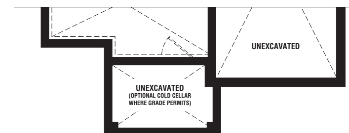
PARTIAL BASEMENT PLAN ELEV. B
