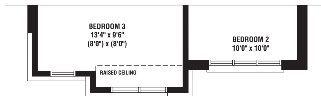
PARTIAL SECOND FLOOR PLAN ELEV. C
