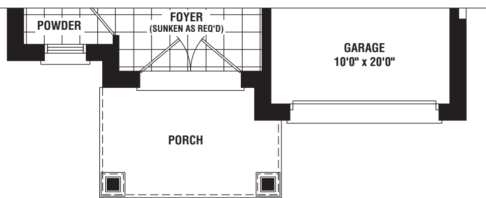
PARTIAL GROUND FLOOR PLAN ELEV. B
