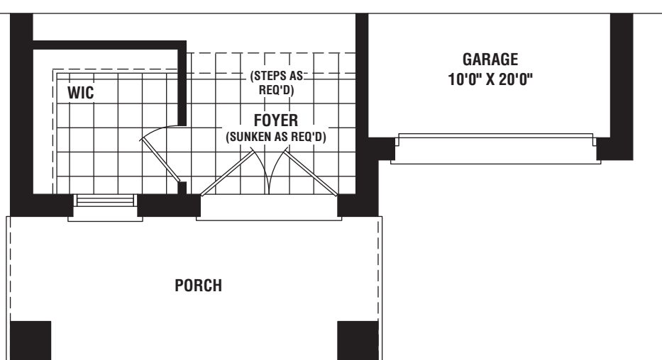
PARTIAL GROUND FLOOR PLAN ELEV. 'C'
