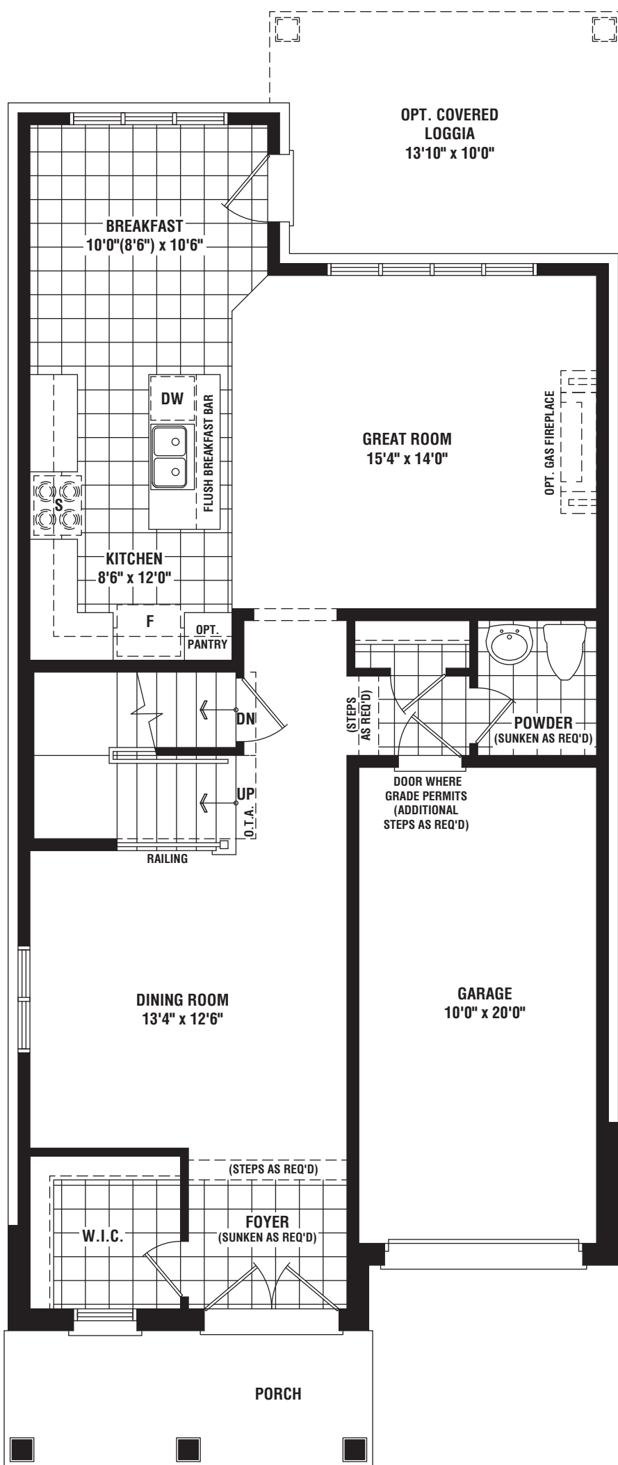
GROUND FLOOR PLAN ELEV. 'A'
