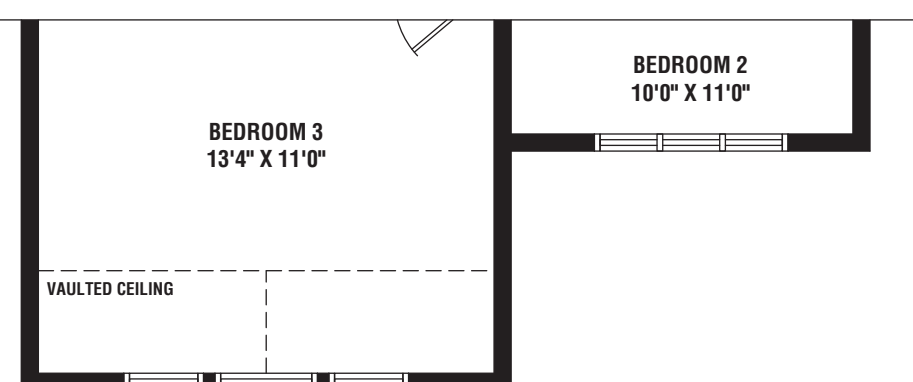
PARTIAL SECOND FLOOR PLAN ELEV. 'B'
