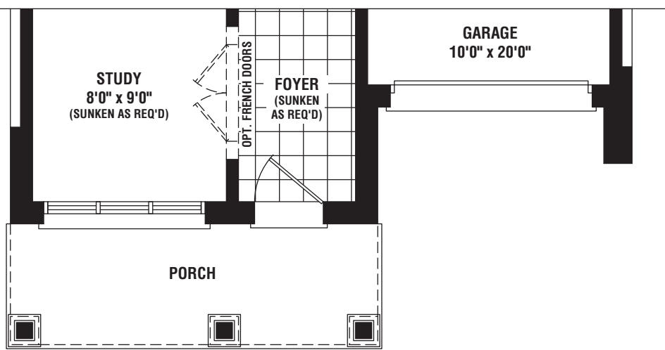
PARTIAL GROUND FLOOR PLAN ELEV. 'B'
