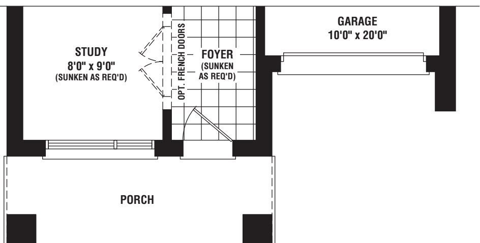
PARTIAL GROUND FLOOR PLAN ELEV. 'C'
