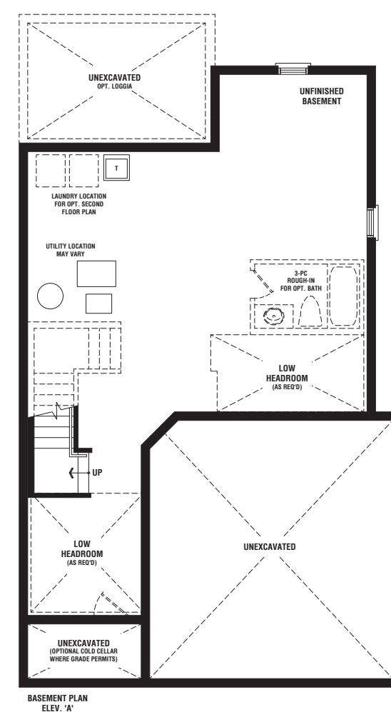
BASEMENT PLAN ELEV. 'A'
