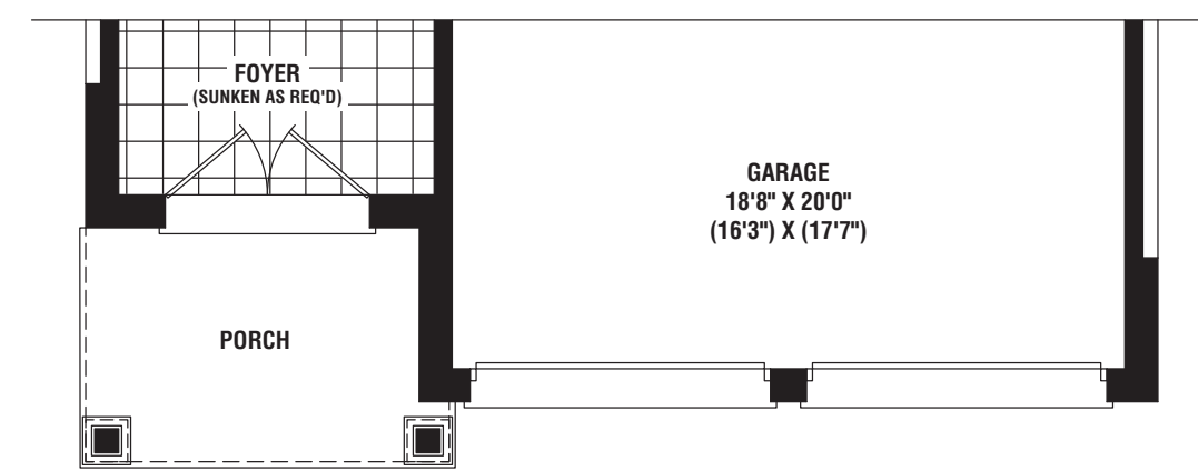
PARTIAL GROUND FLOOR PLAN ELEV. 'B'
