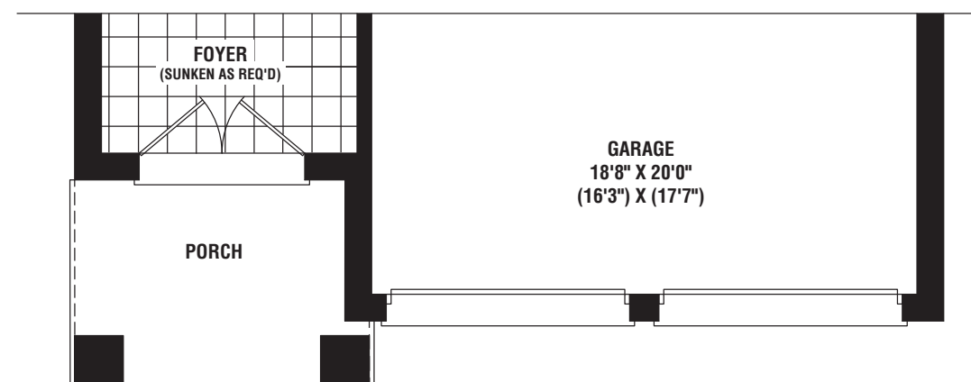
PARTIAL GROUND FLOOR PLAN ELEV. 'C'
