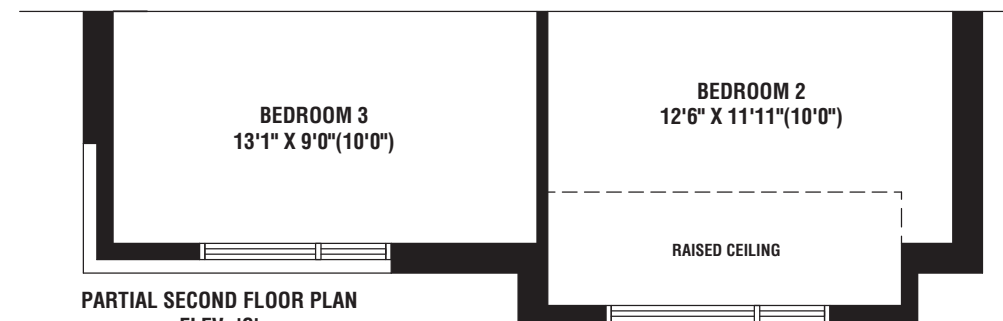
PARTIAL SECOND FLOOR PLAN ELEV. 'B'
