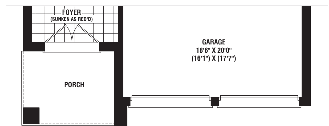
PARTIAL GROUND FLOOR PLAN ELEV. 'C'
