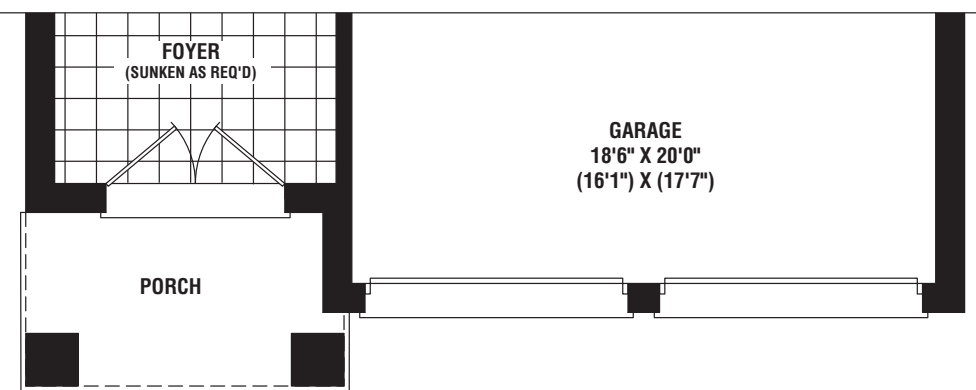
PARTIAL GROUND FLOOR PLAN ELEV. 'C'
