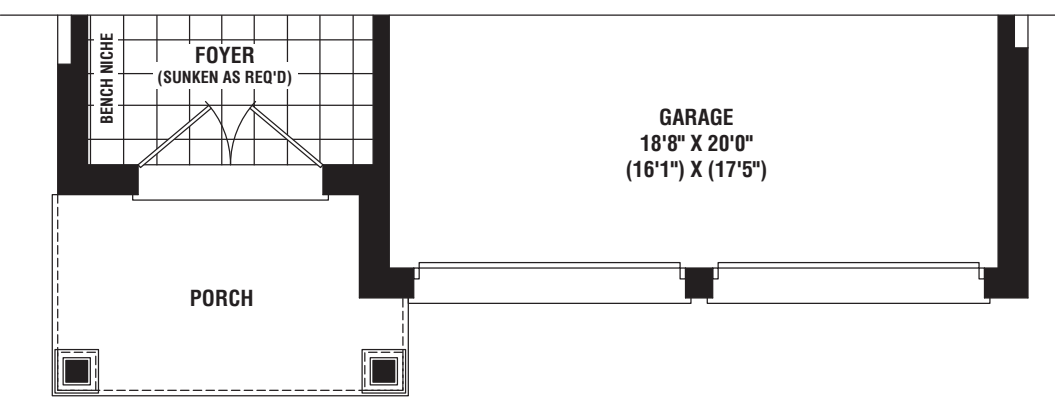
PARTIAL GROUND FLOOR PLAN ELEV. 'B'
