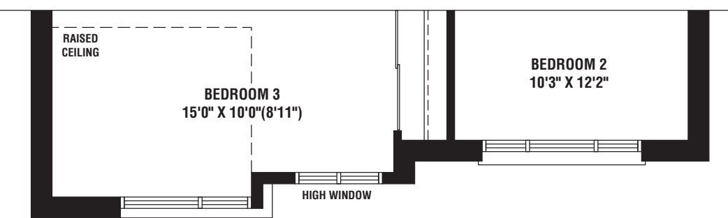
PARTIAL SECOND FLOOR PLAN ELEV. 'C' 8' CEILING
