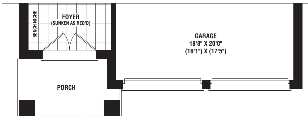
PARTIAL GROUND FLOOR PLAN ELEV. 'C'
