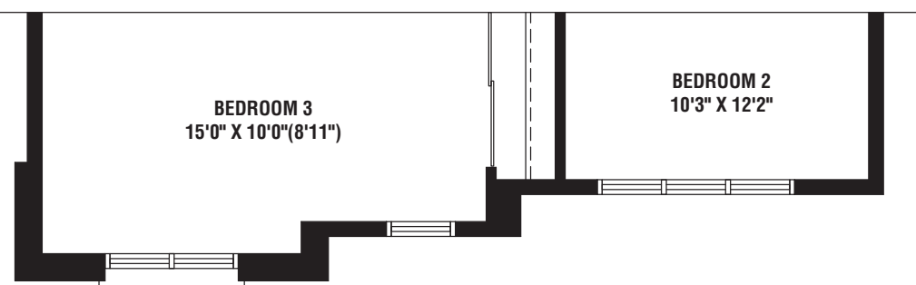
PARTIAL SECOND FLOOR PLAN ELEV. 'B'
