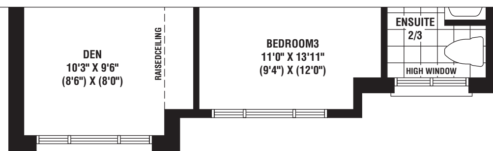
PARTIAL SECOND FLOOR PLAN ELEV. 'C'
