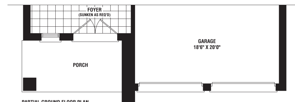
PARTIAL GROUND FLOOR PLAN ELEVATION 'C'
