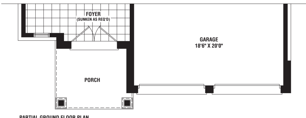
PARTIAL GROUND FLOOR PLAN ELEVATION 'B'
