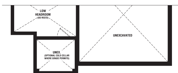
PARTIAL BASEMENT PLAN ELEVATION 'B'
