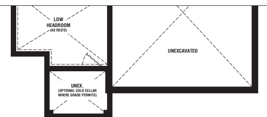
PARTIAL BASEMENT PLAN ELEV. 'B'
