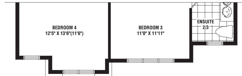
PARTIAL SECOND FLOOR PLAN ELEV. 'B'
