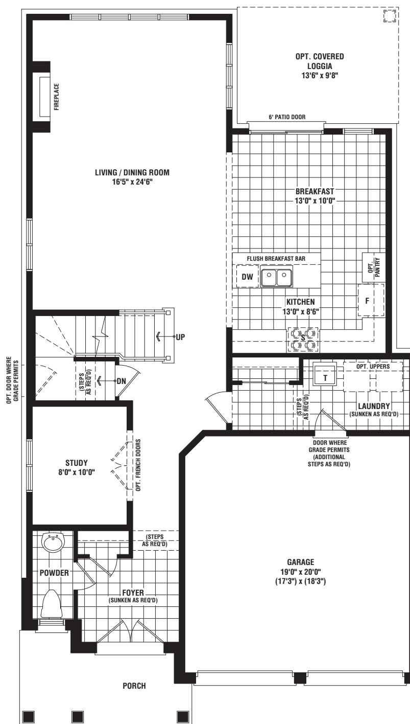
ALT. GROUND FLOOR PLAN ELEV. 'A'
