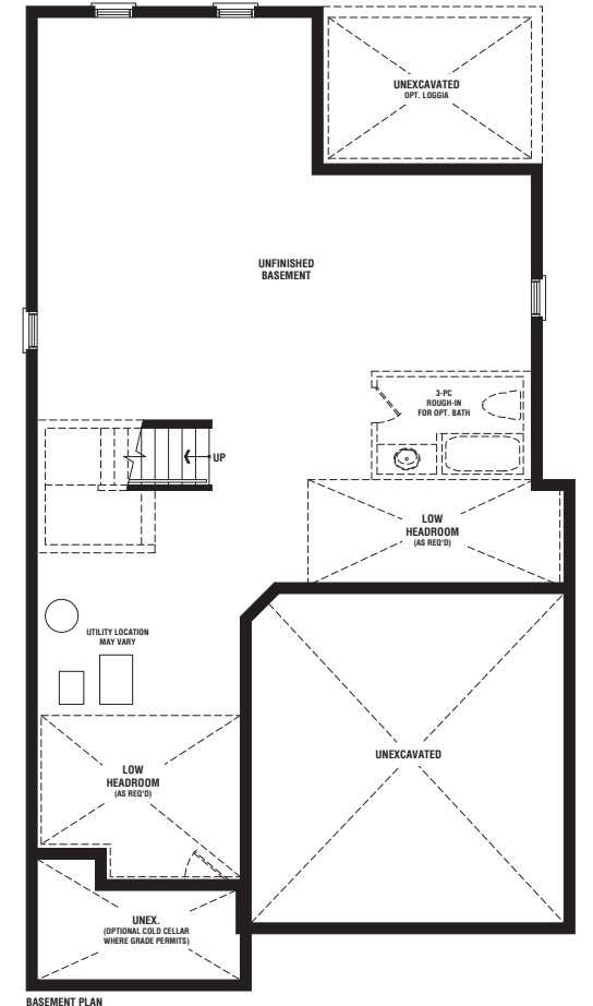
BASMENT PLAN ELEV. 'A'
