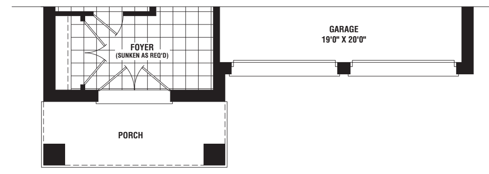
PARTIAL GROUND FLOOR PLAN ELEV. 'C'
