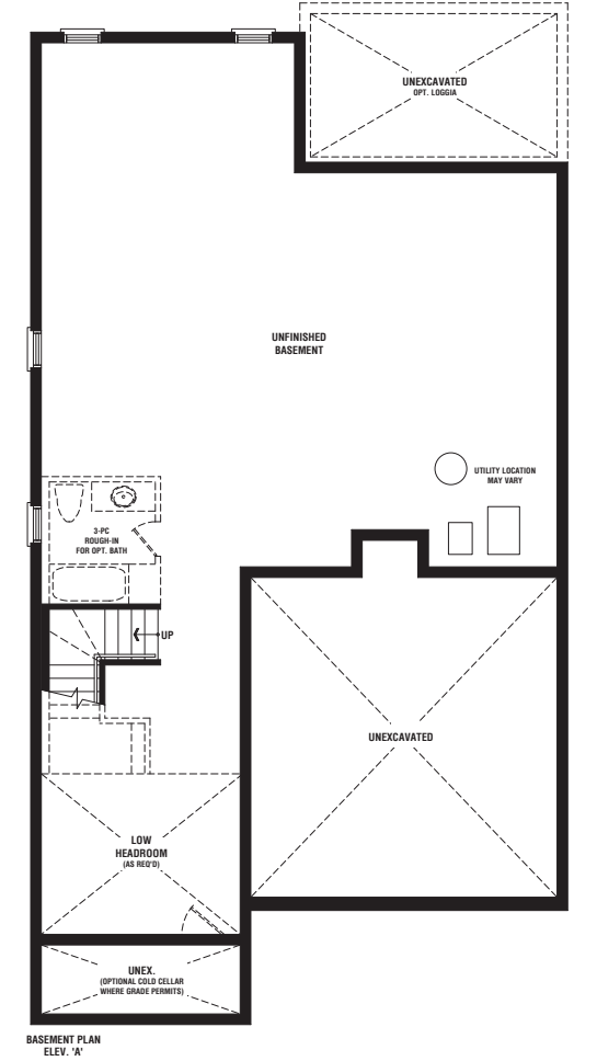
BASEMENT PLAN ELEV. 'A'
