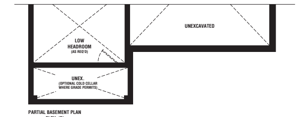
PARTIAL BASEMENT PLAN ELEV. 'B'
