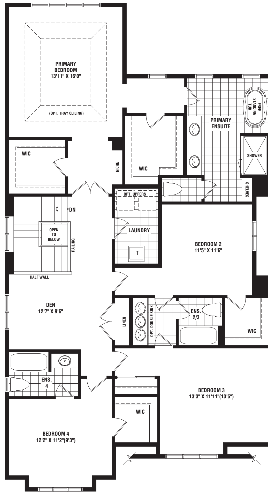
SECOND FLOOR PLAN ELEV. 'A'
