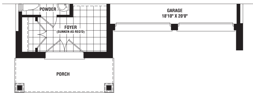
PARTIAL GROUND FLOOR PLAN ELEV. 'B'
