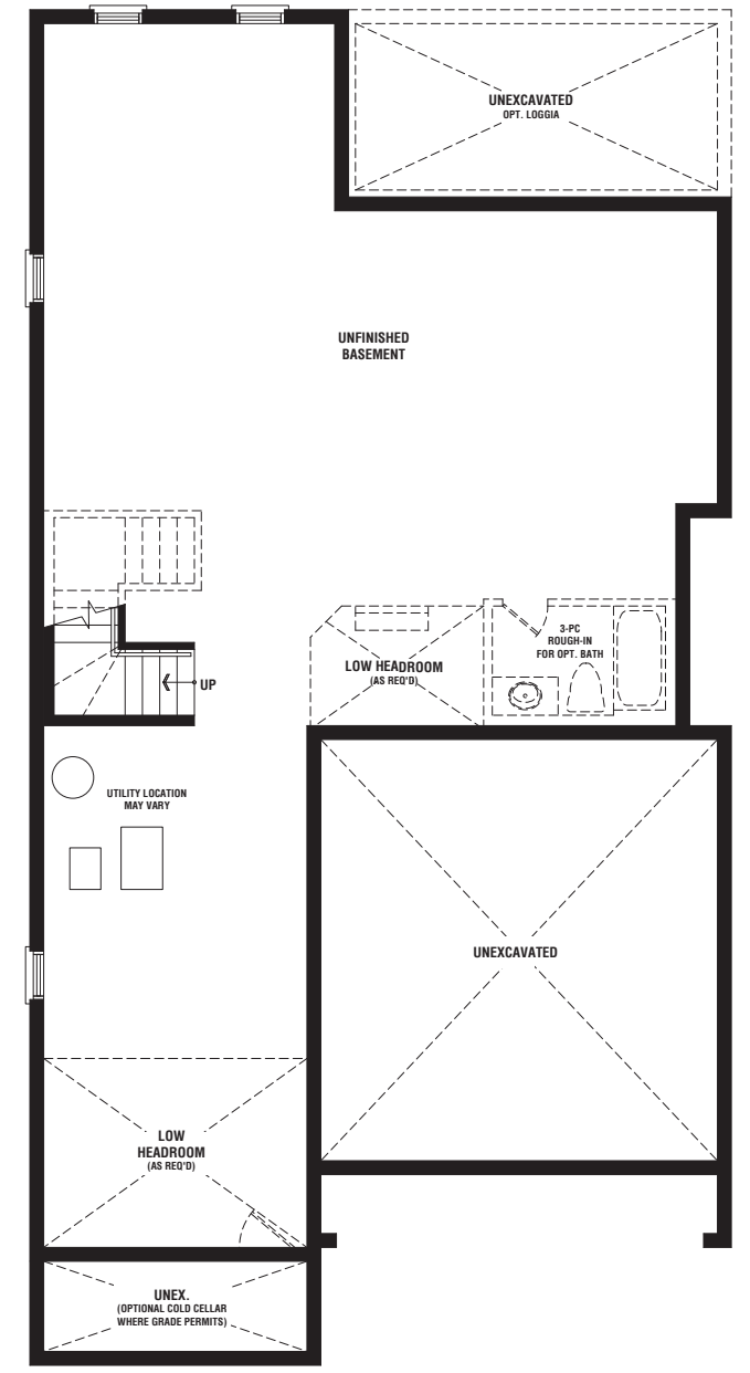
BASEMENT PLAN ELEV. 'A'
