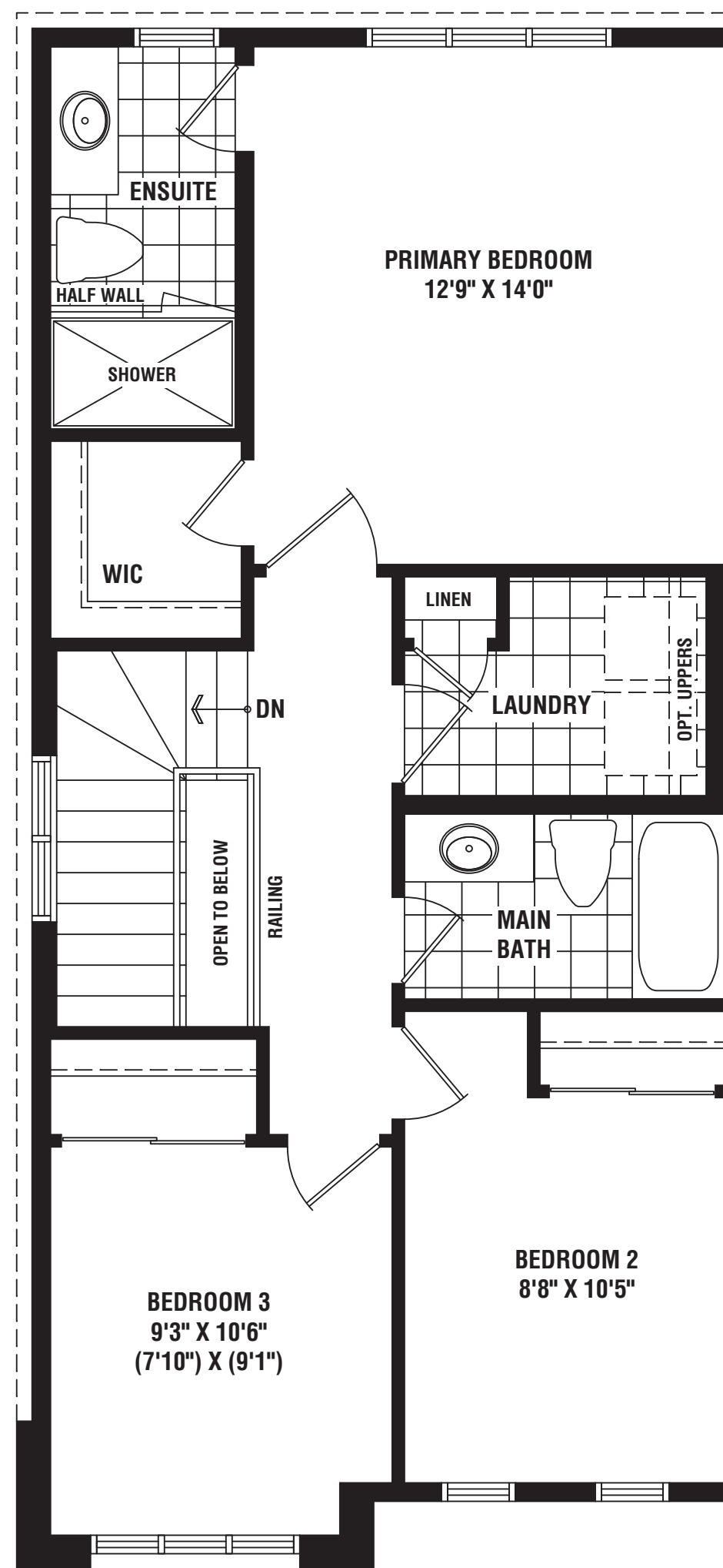
SECOND FLOOR PLAN ELEV. 'B3'
