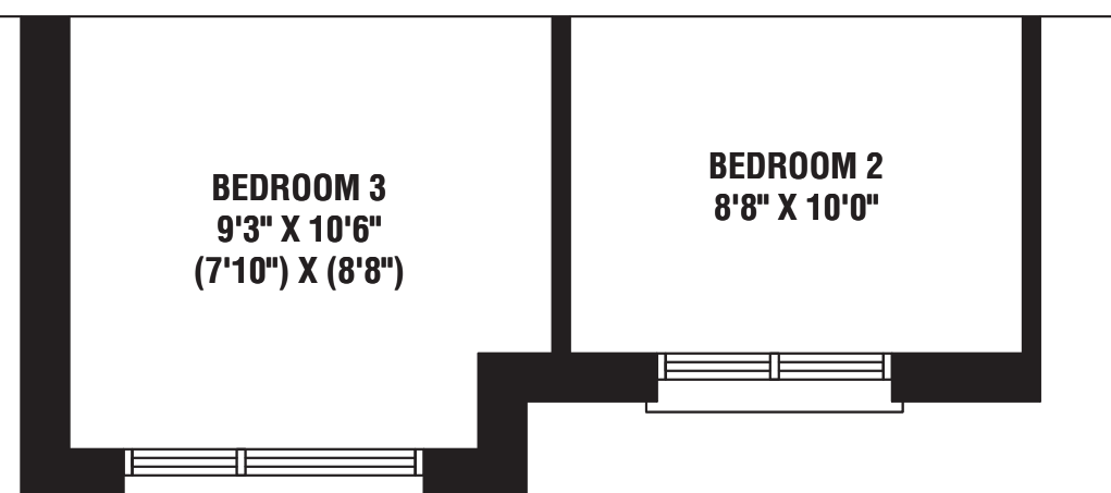
PARTIAL SECOND FLOOR PLAN ELEV. 'C3'
