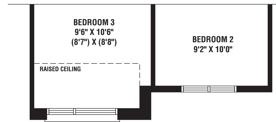
PARTIAL SECOND FLOOR PLAN ELEV. 'C'
