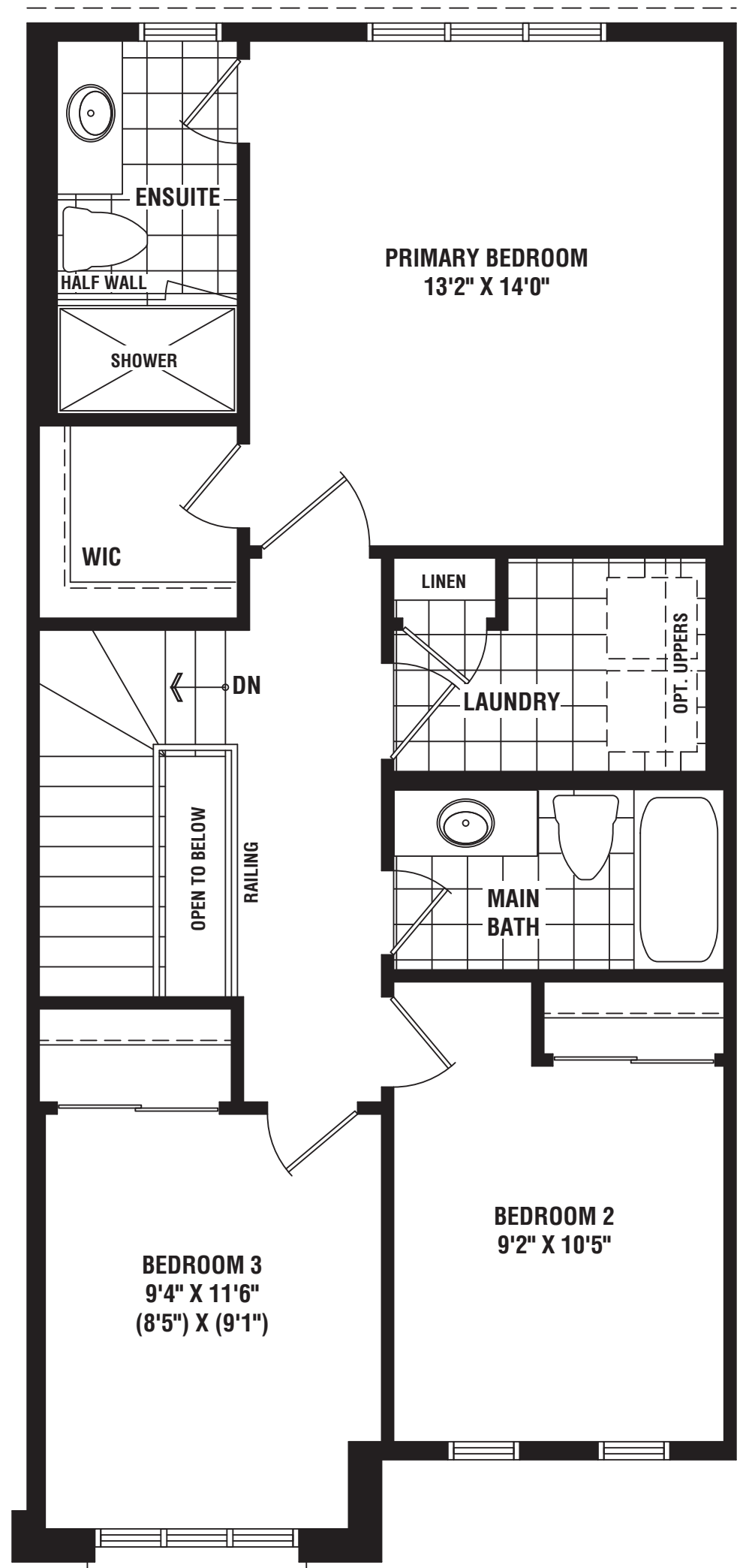
SECOND FLOOR PLAN ELEV. 'B1'
