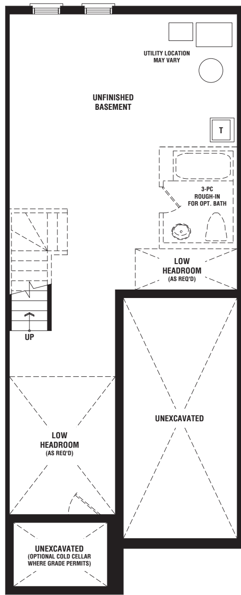
BASEMENT PLAN ELEV. 'B1'
